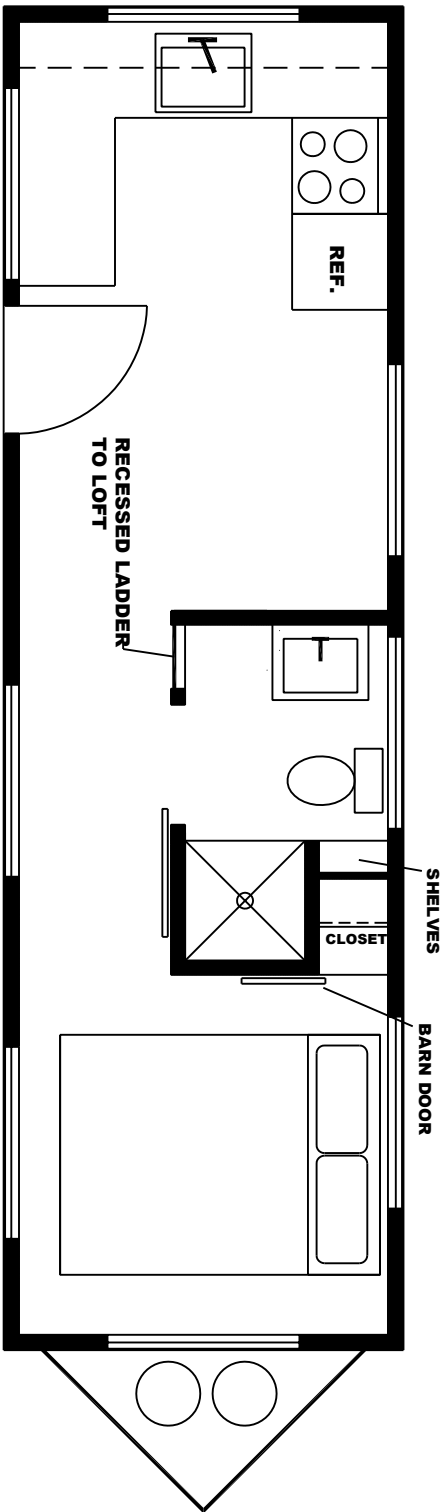
JUDE 8'-6" X 20'
